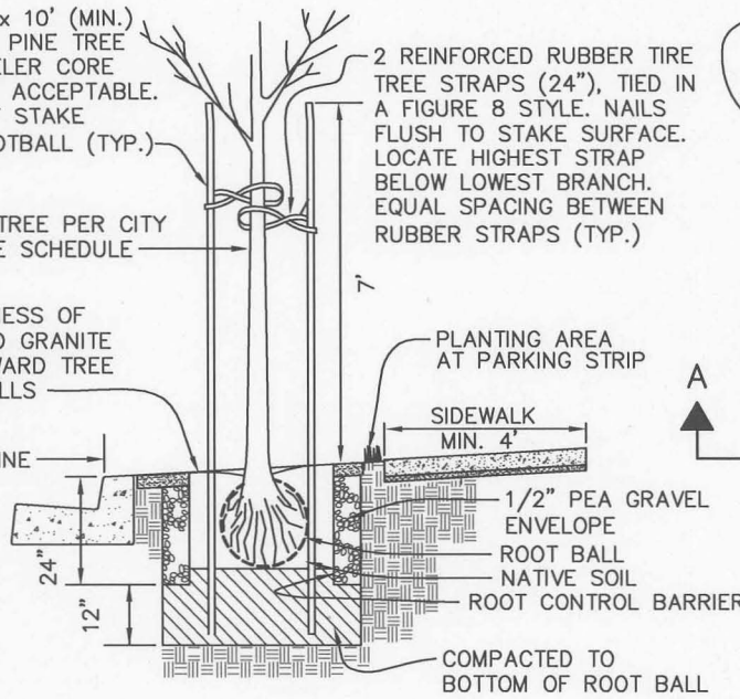
STAKING DETAIL
