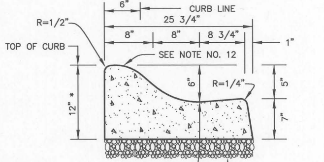
STANDARD ROLL CURB
