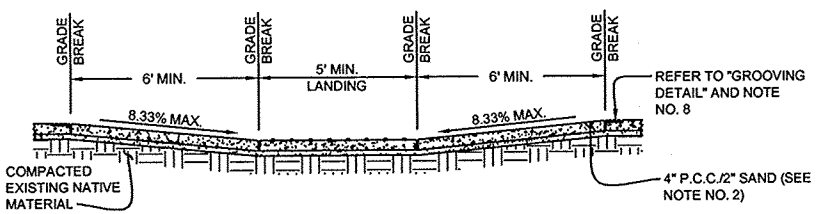
SECTION E-E
