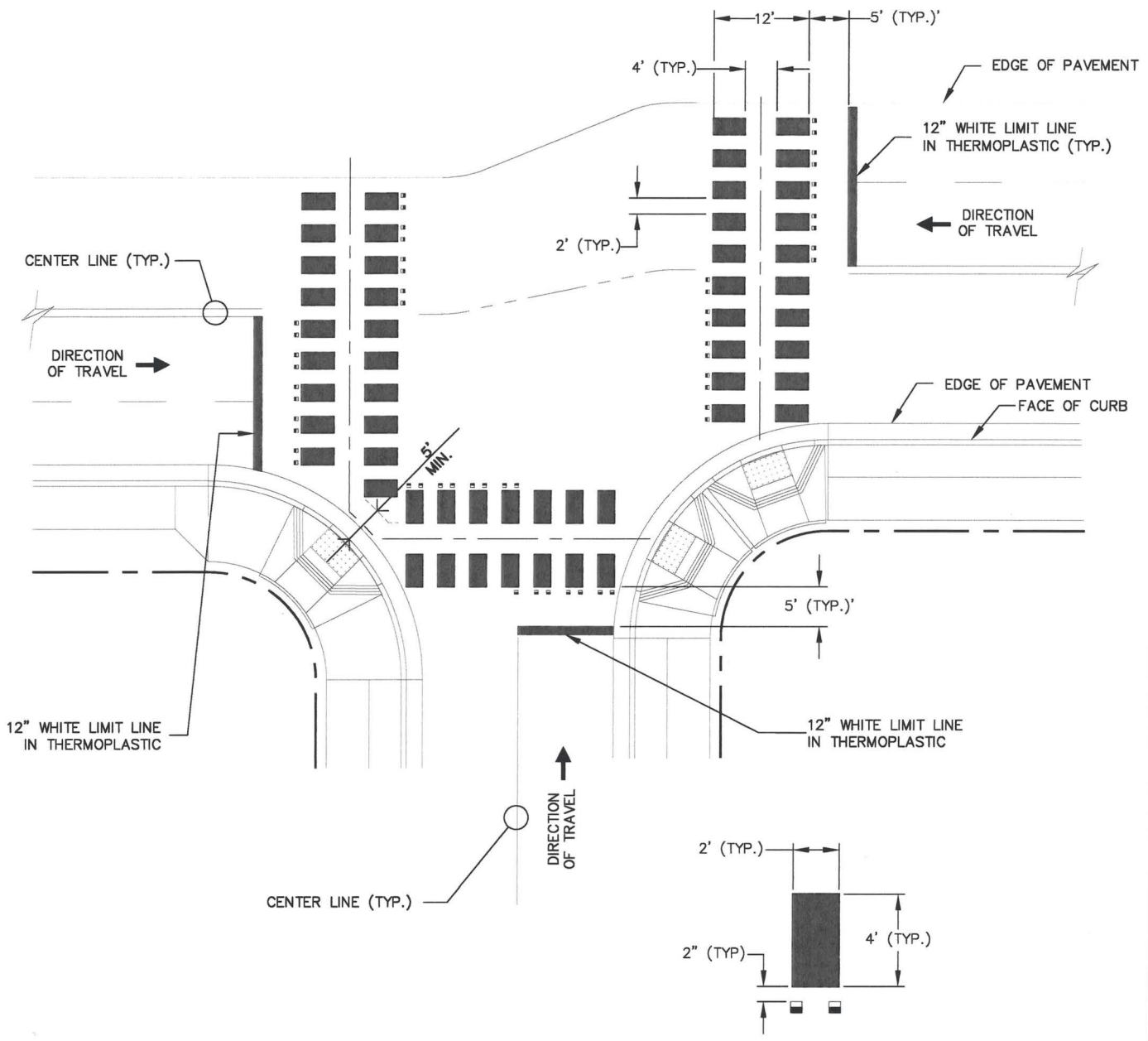
TYPE G RAISED PAVEMENT MARKER DETAIL
