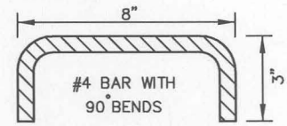
DETAIL OF DOWEL
