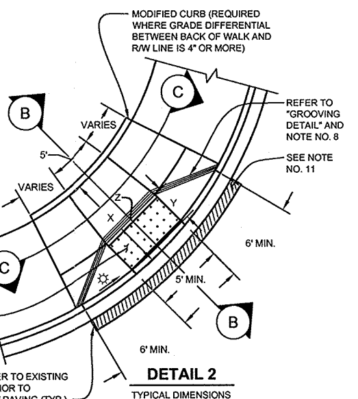
TYPE "B" ADA PEDESTRIAN ACCESS RAMP ALTERNATE LOCATION
