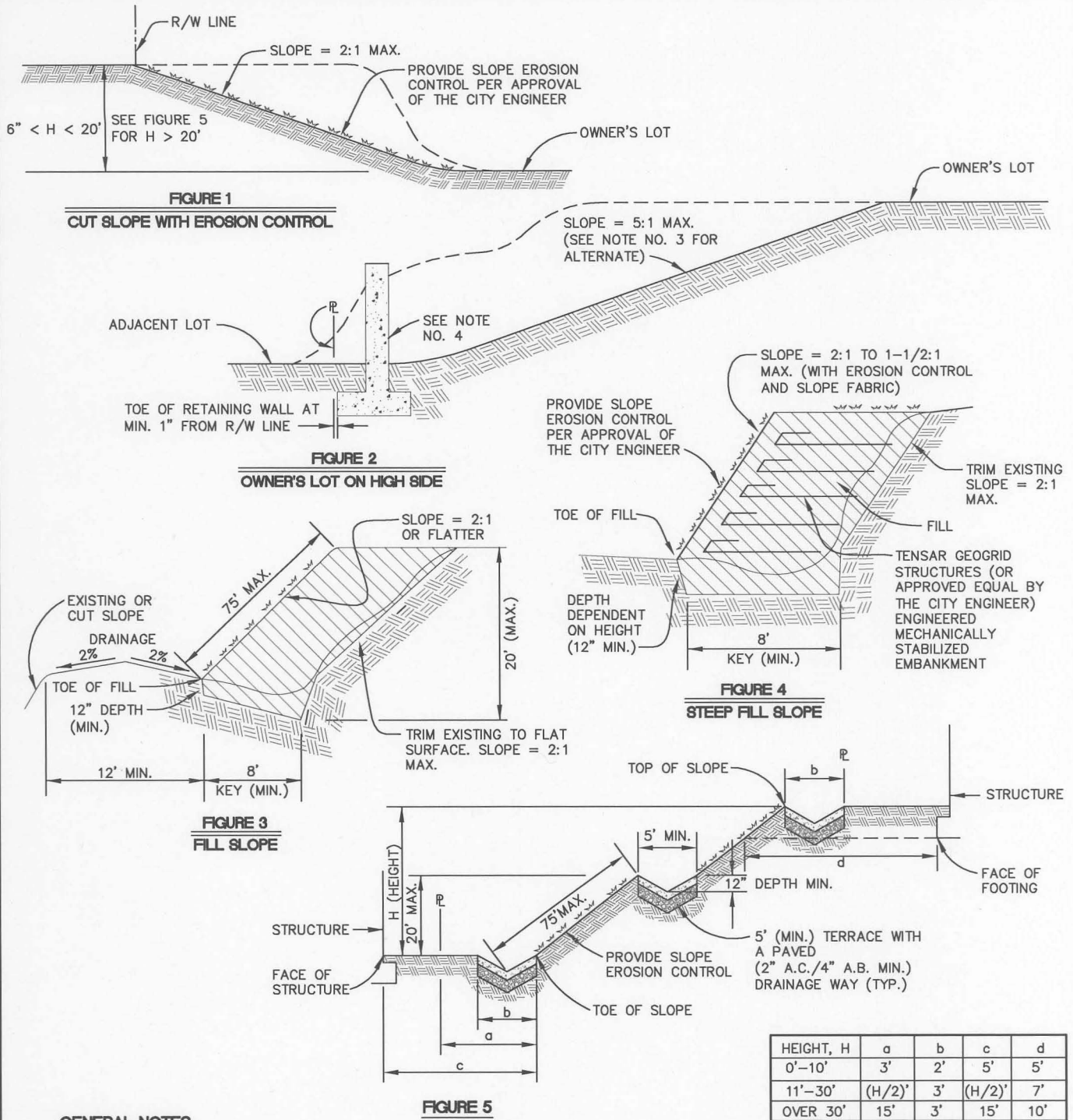
CUT AND FILL SETBACKS
