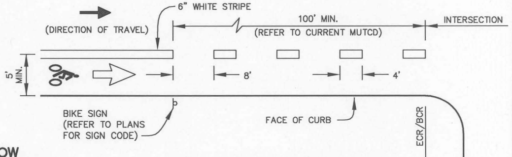
DETAIL "C"
