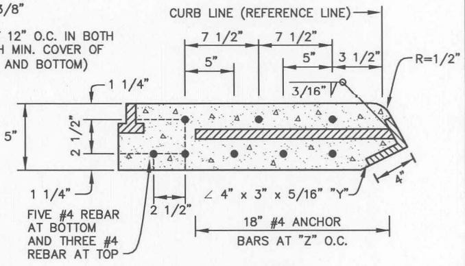
DETAIL OF REINFORCEMENT
