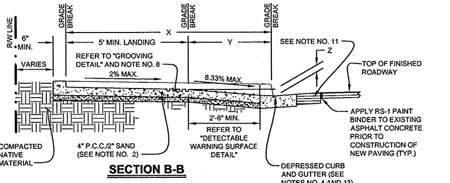
DETAIL 2 TYPICAL DIMENSIONS
