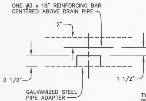
PROFILE
