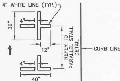
PARKING TEE DETAIL
